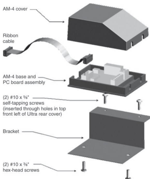
Figure 1 AM4 assembly
