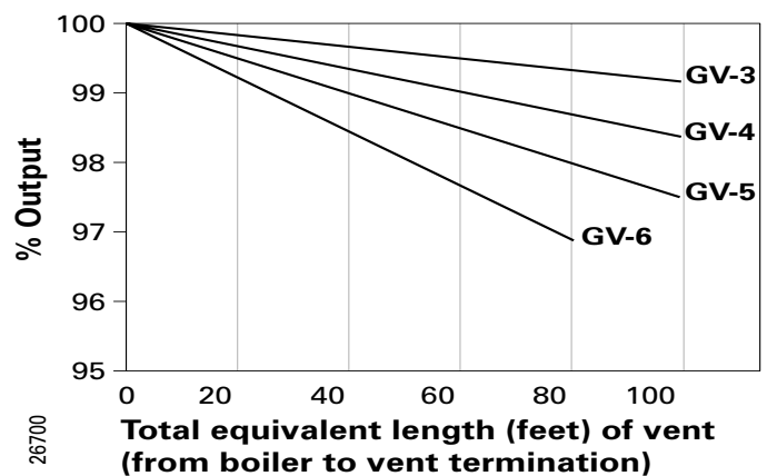
Figure 2 Boiler output
