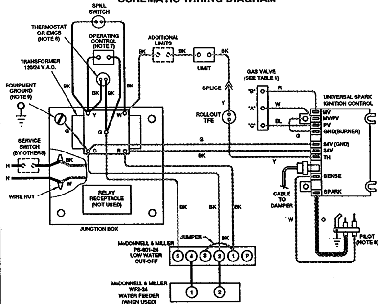
SCHEMATIC WIRING DIAGRAM
