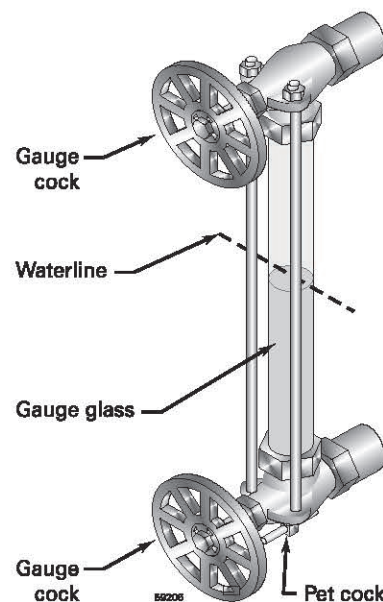
Figure 9 Gauge glass
