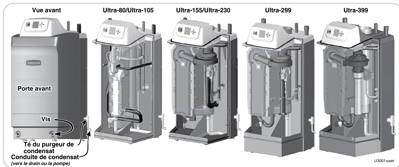
Figure 3 Emplacements des composants Ultra
