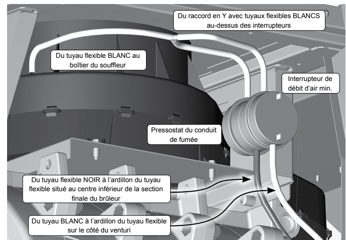
Figure 73 Pressostats
