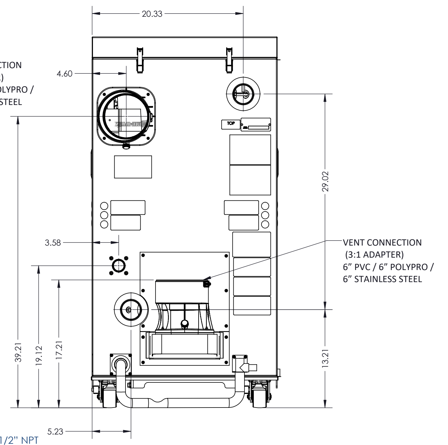
BACK VIEW
