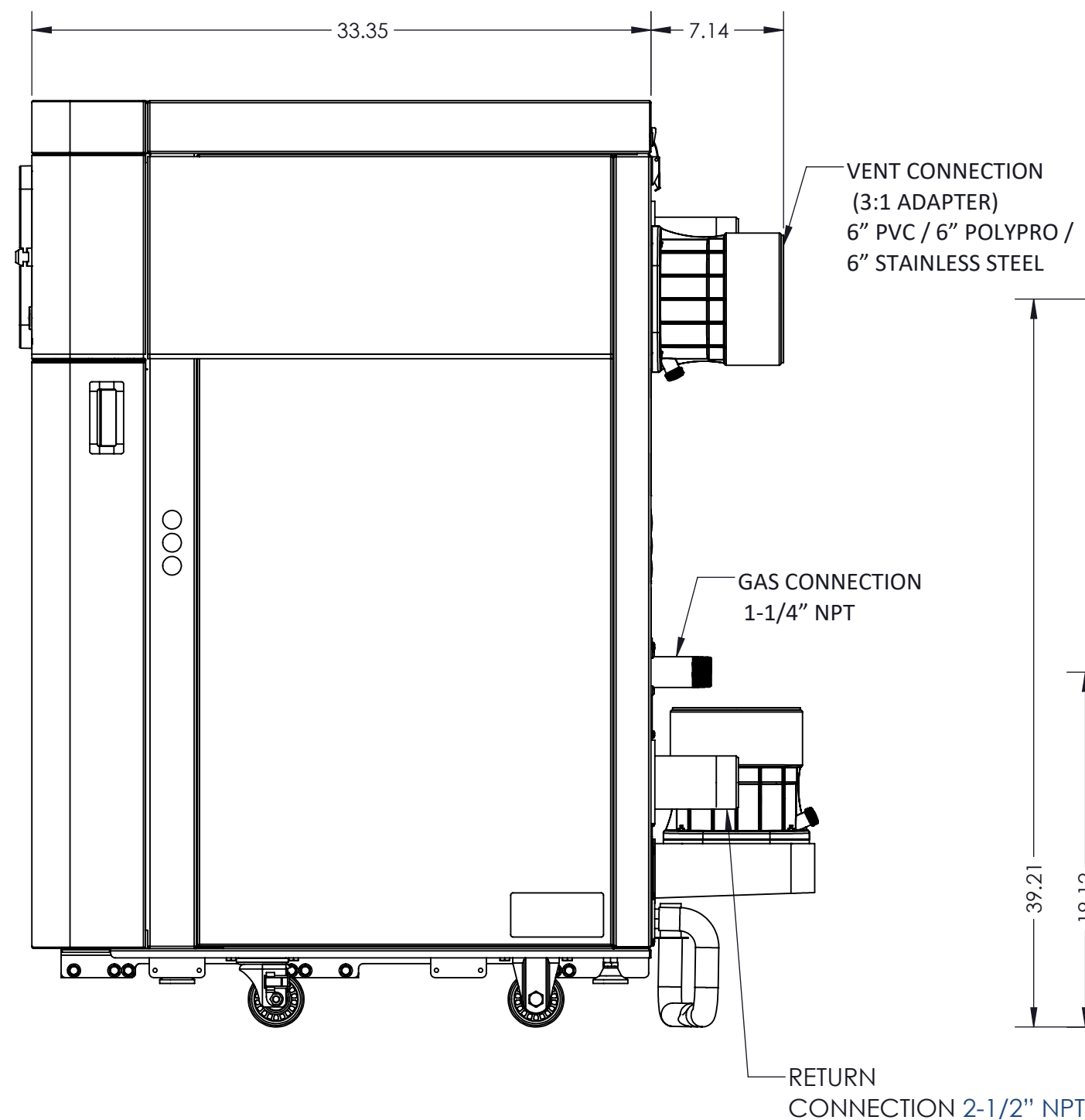
SIDE VIEW
