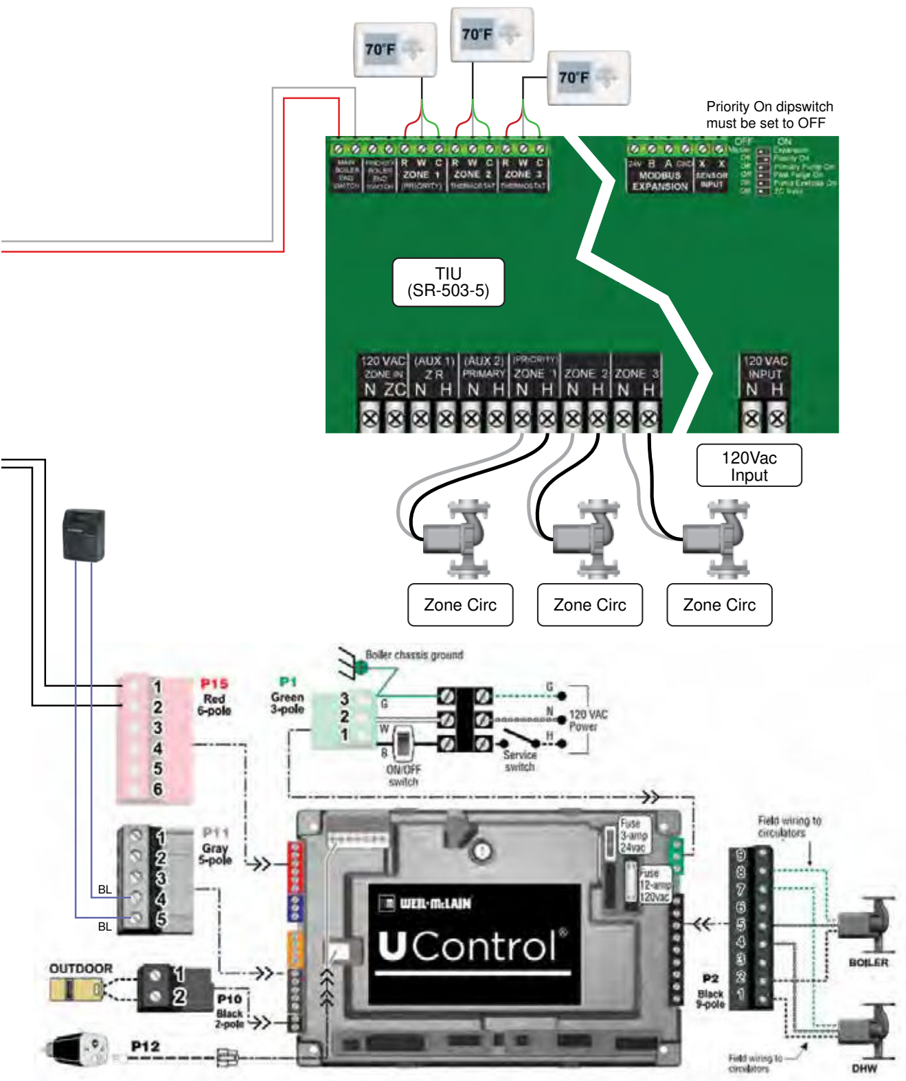
Figure 30 Application B3: Multi-zone Space Heating boiler only DHW Application Wiring
