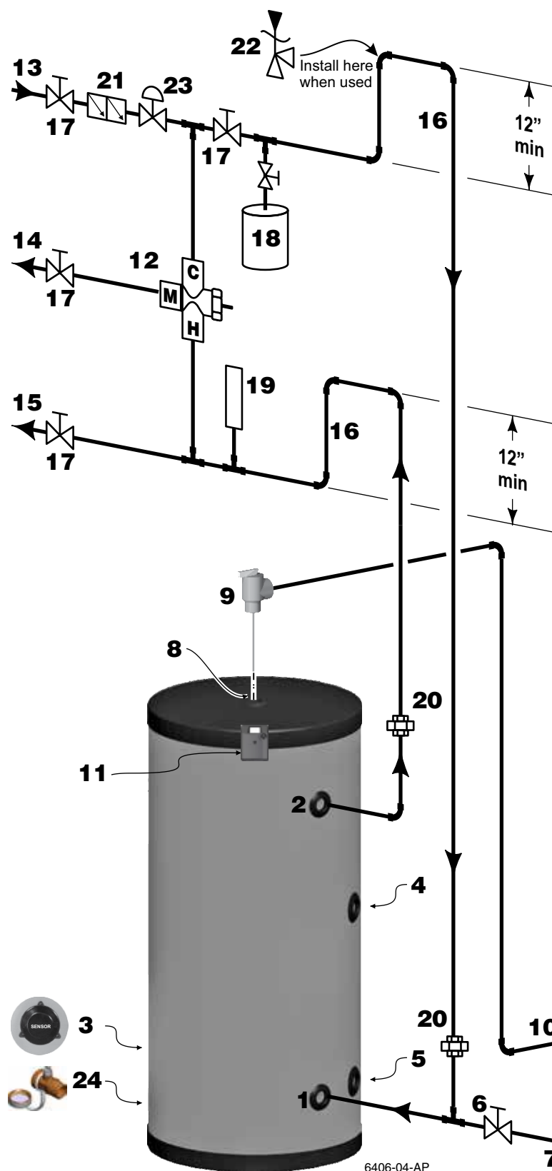
Figure 2 DHW piping
