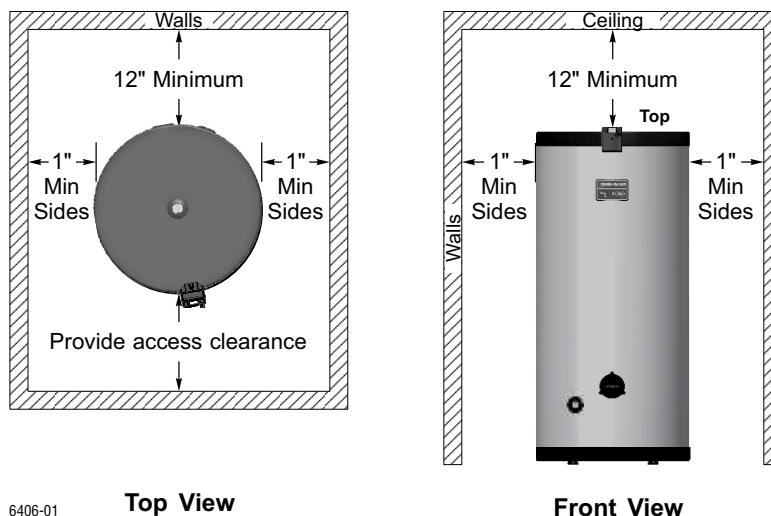
Figure 1 Clearance recommendations
