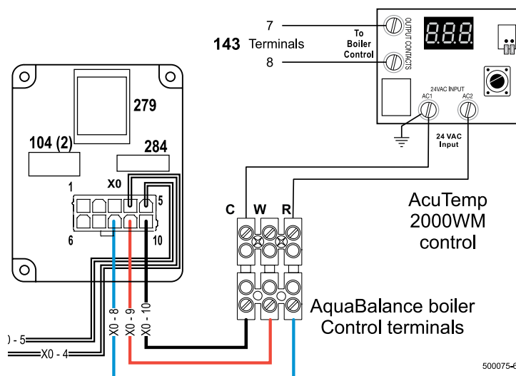
Figure 18 Wiring tank control to the AquaBalance® boiler control.
