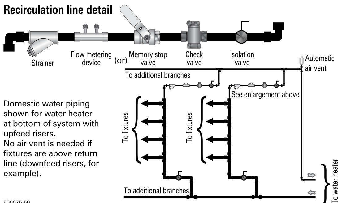
Figure 5 Recirculation components
