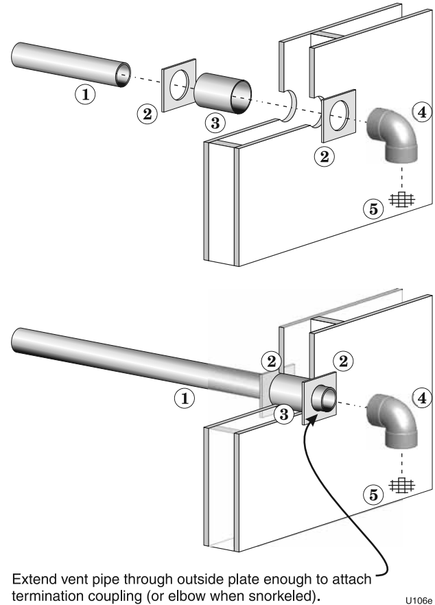
Figure 29 DIRECT EXHAUST — Sidewall — termination assembly — all parts by installer
