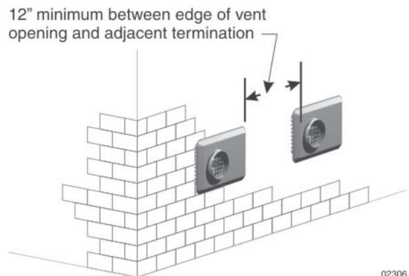
Figure 8 Multiple vent/air terminations (must also comply with other clearances for individual terminations)
