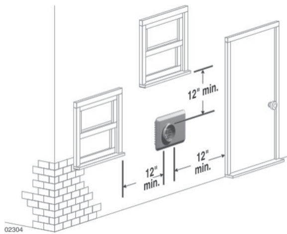
Figure 6 Clearance to gravity air inlets
