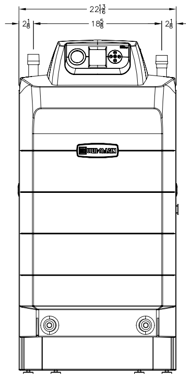
FRONT
