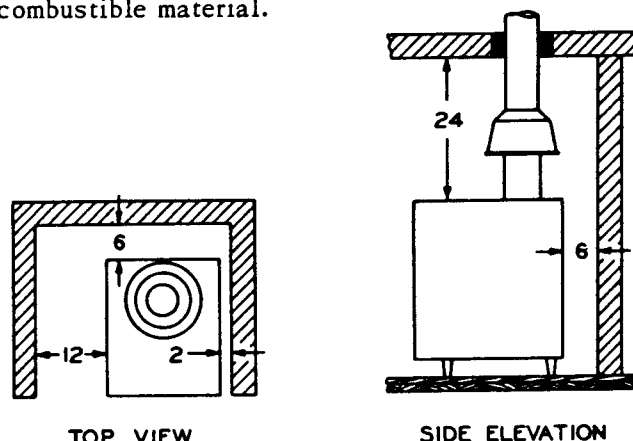
MINIMUM CLEARANCE FOR ALCOVE INSTALLATIONS
