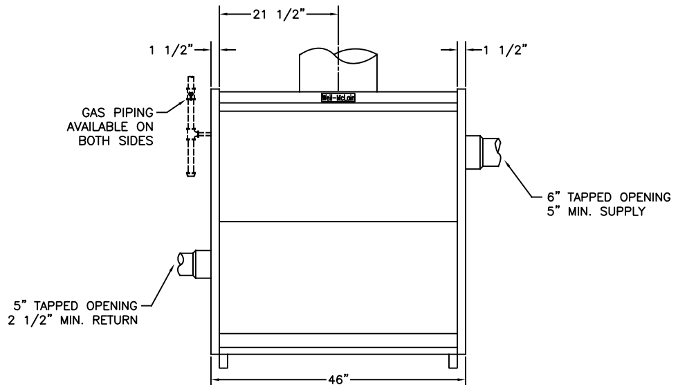
FRONT
