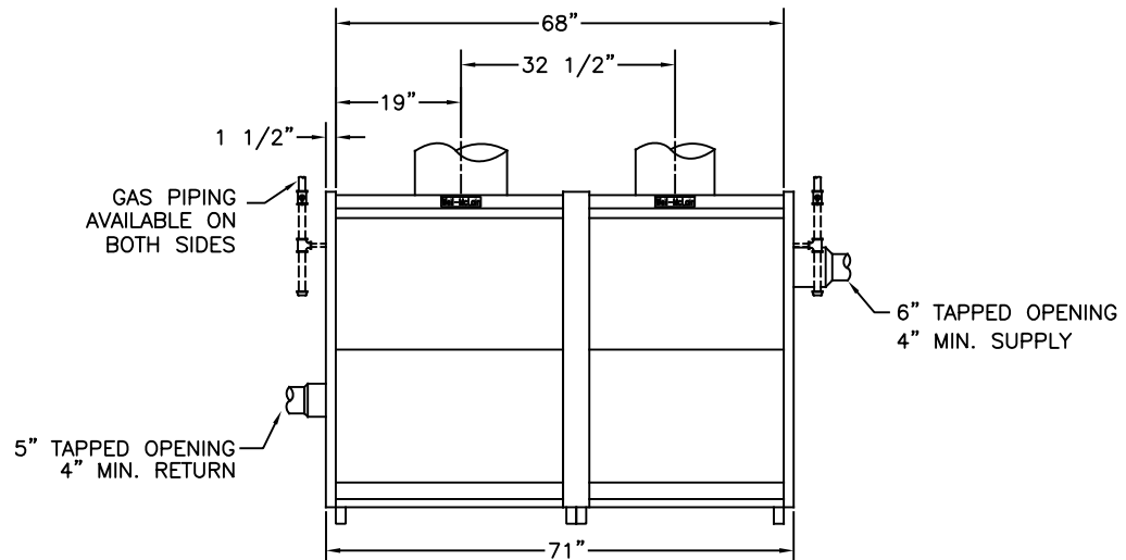
FRONT
