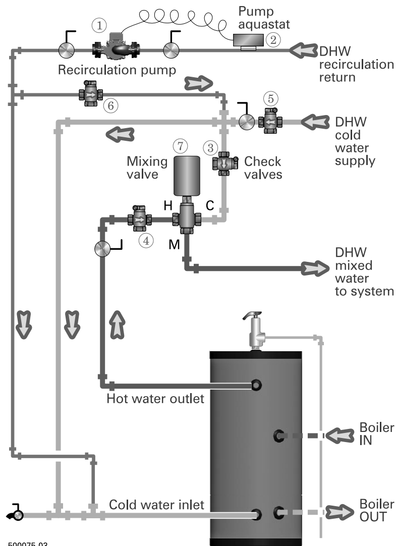
Figure 6 Recirculation piping
