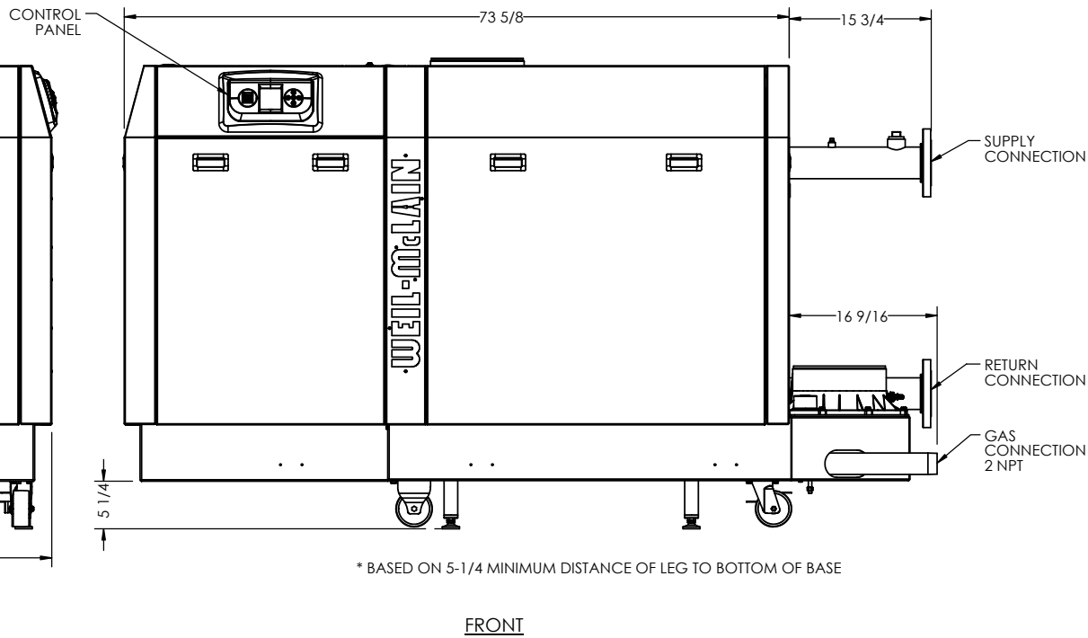
SLIMFIT SF2000 RH BOILER
