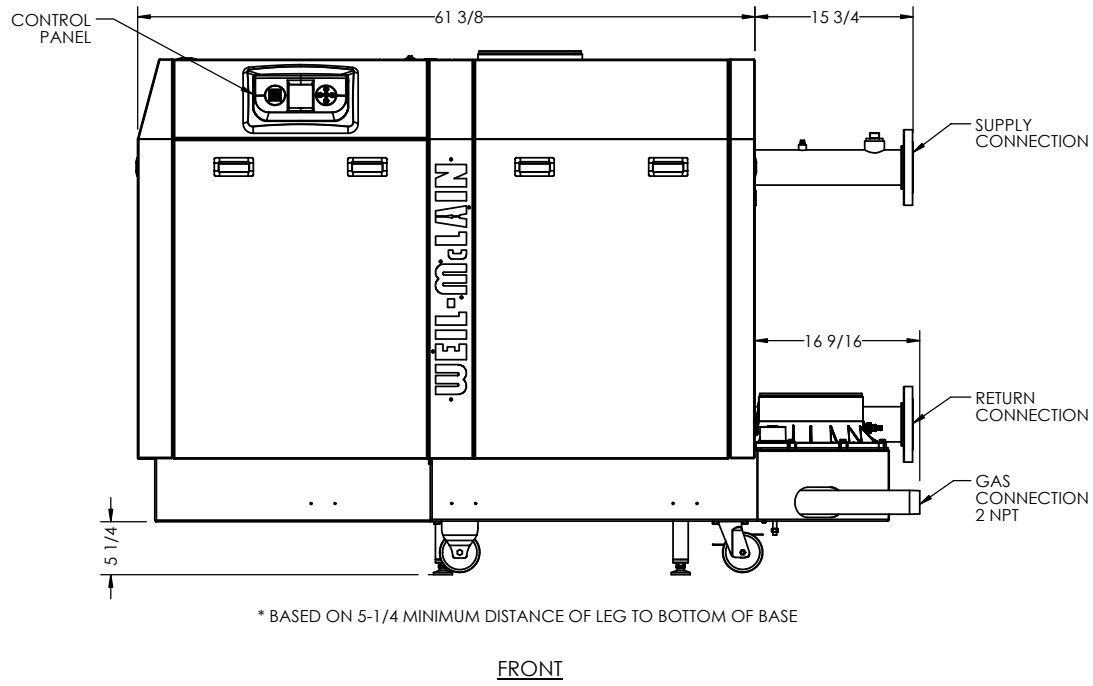
SLIMFIT SF1000 RH BOILER
