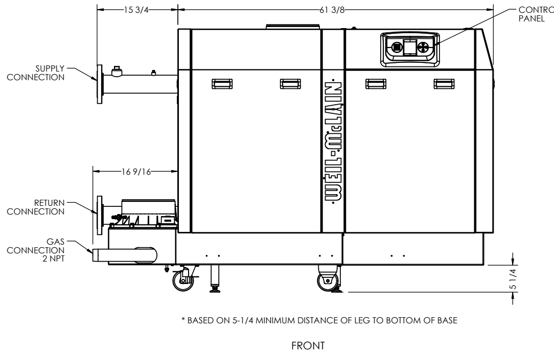
SLIMFIT SF1500 LH BOILER
