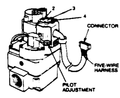
36C84 GAS VALVE FIGURE 7
